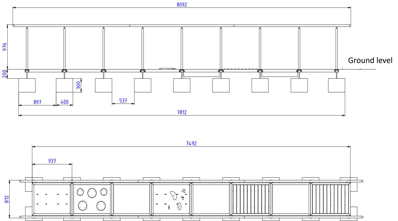
Fig. Dimensions of the device with a length of 8 sections
